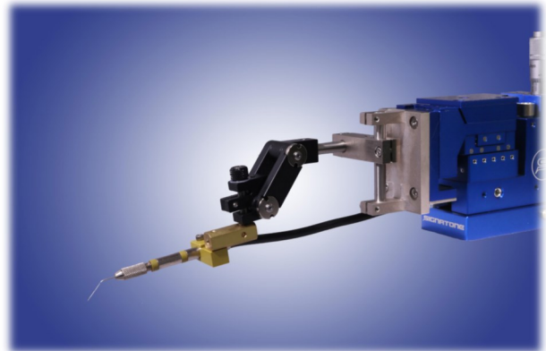
Figure 2 HVP-CX-3 mounted on a SP100 positioner
